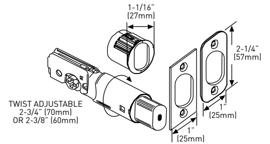
6-IN-1 ADJUSTABLE DEADBOLT LATCH
