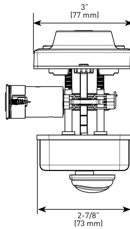
CONCIERGE 200 TOP VIEW
