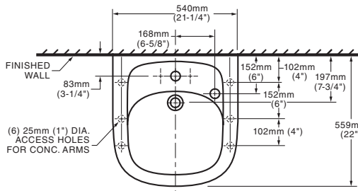
0955.123EC Center Hole With Extra Right Hand Hole
