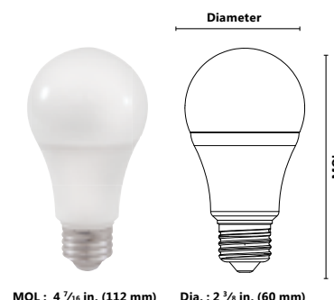
MOL : 4 7/16 in. (112 mm) Dia. : 2 1/8 in. (60 mm)
