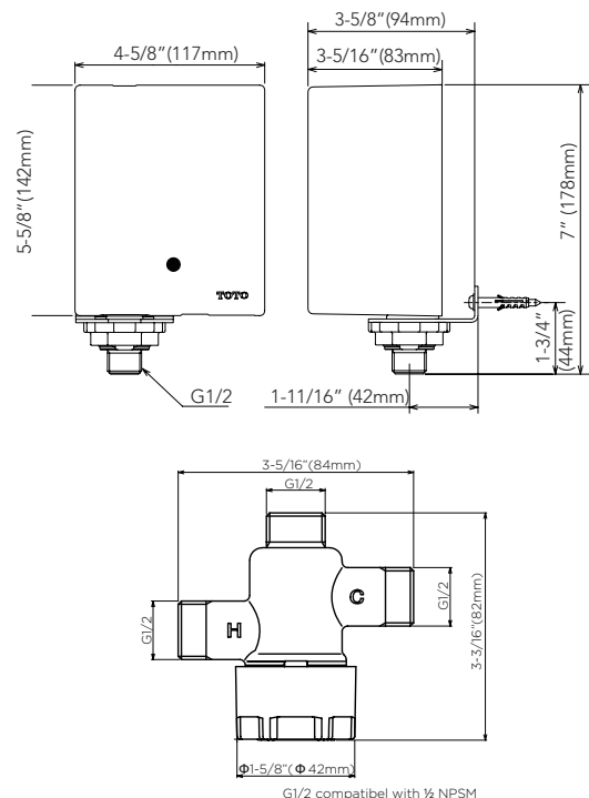
Thermostatic Mixing Valve (TLT10)
