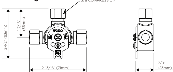
Hot/Cold Mixing Tee (TLM10)
