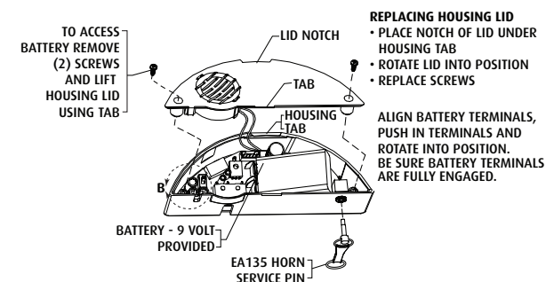
VIEW SHOWING BATTERY REPLACEMENT
