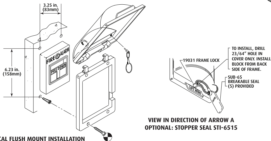
TYPICAL FLUSH MOUNT INSTALLATION
