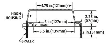
ALL HORN MODELS SIDE VIEW
