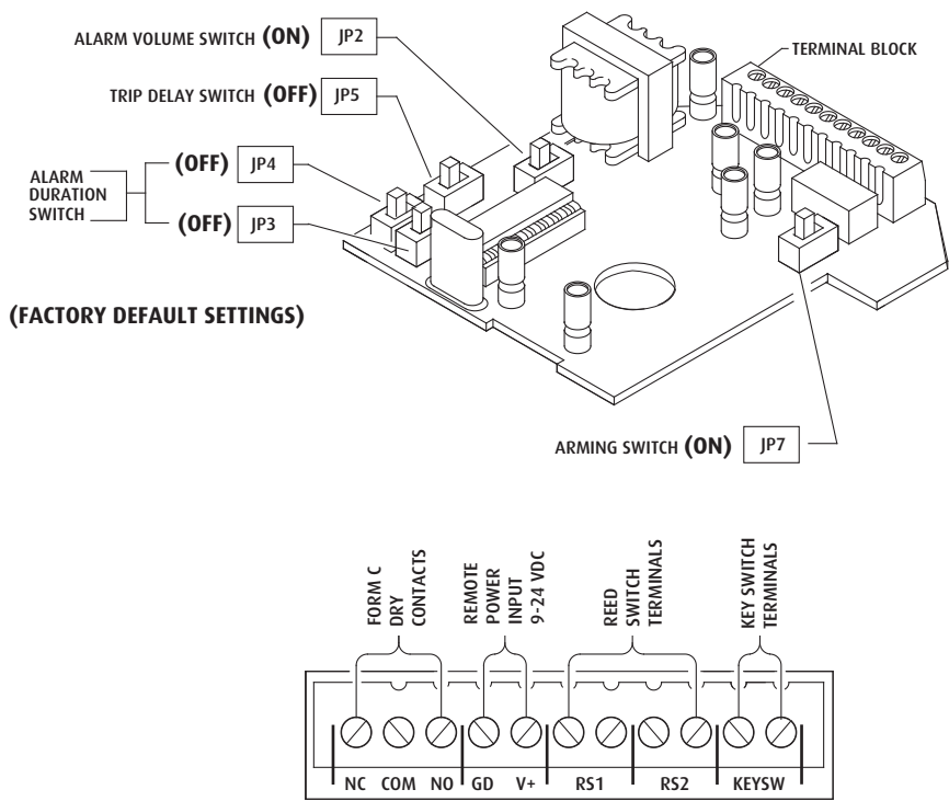
TERMINAL BLOCK WIRING CONNECTIONS
