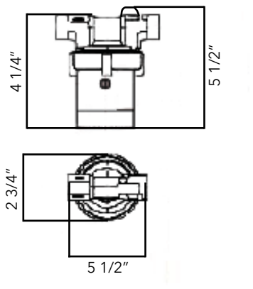
UltraCirc Pump Housing (Union with Ball & Check Valve)
