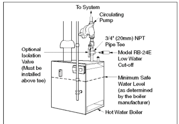
In a Pipe Tee Above the Boiler
