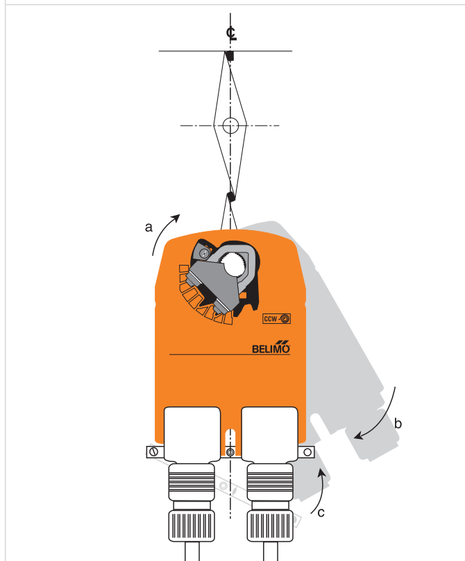
FIGURE B – Standard Mounting (Dimensions in Inches [mm])
