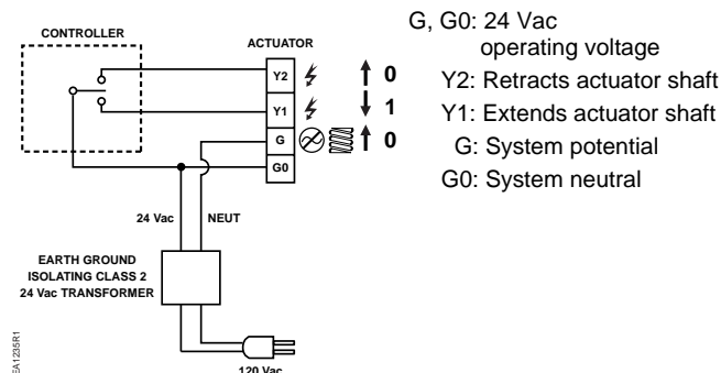
Figure 7. SSC81.5U Floating Control SR Hot-Switch.
