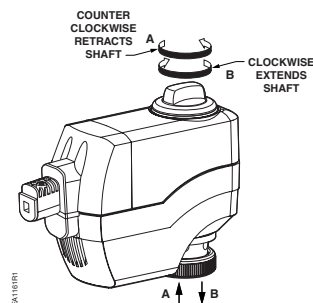
Figure 4. Manual Override.
