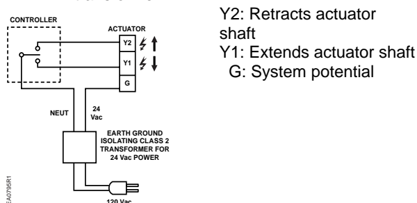
Figure 6. SSC81U NSR Floating Control.
