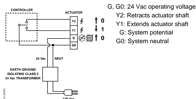
Figure 8. SSC81.5U Floating Control SR Neutral Switching Applications.
